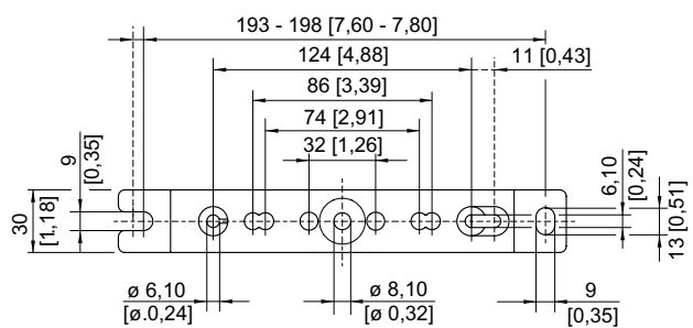
Mounting rail
